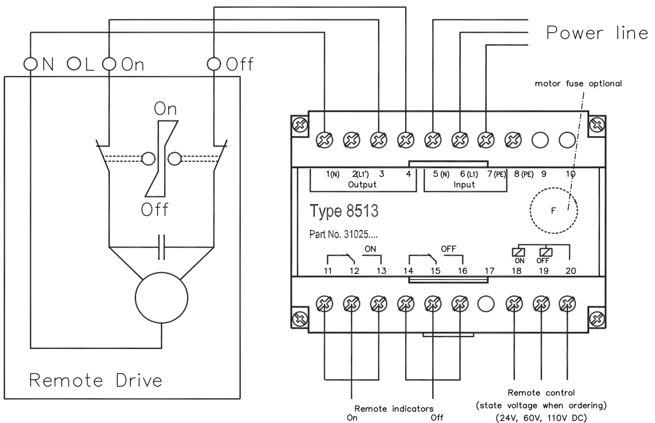
wiring diagram
