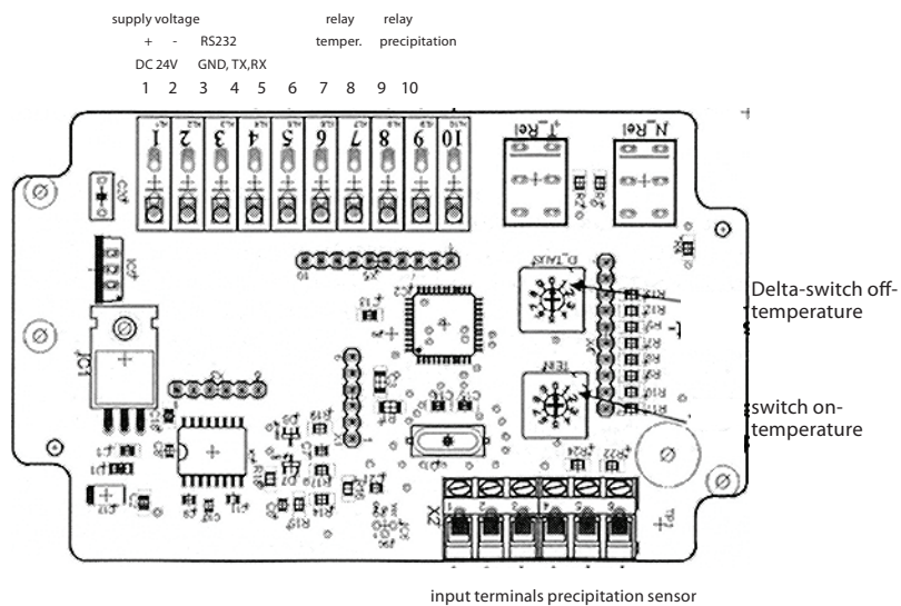
View without cover (PCB side)
