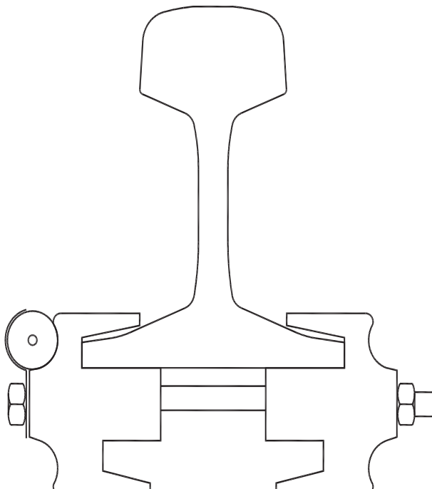
Rail Mounting Fixture, part no. 110404
